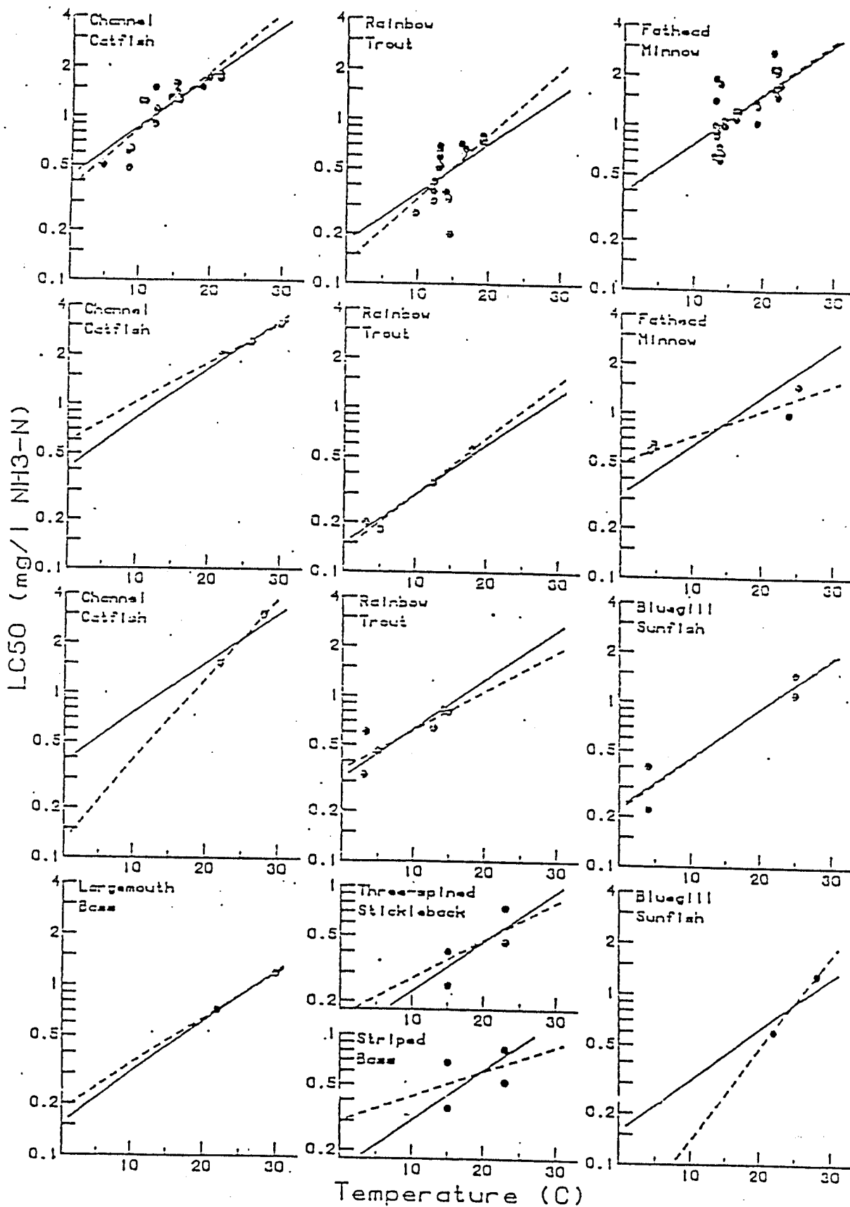
Figure 2. Acute \text{NH}_3 toxicity at different temperatures (data from Cary 1976, Thurston and Russo 1983, Thurston et al. 1983, Colt and Tchobanoulous 1976, Ministry of Technology 1968, Reinbold and Pescitelli 1982, Roseboom and Richey 1977, Hazel et al. 1971). Dashed lines indicate individual regressions; solid lines indicate pooled regression.
