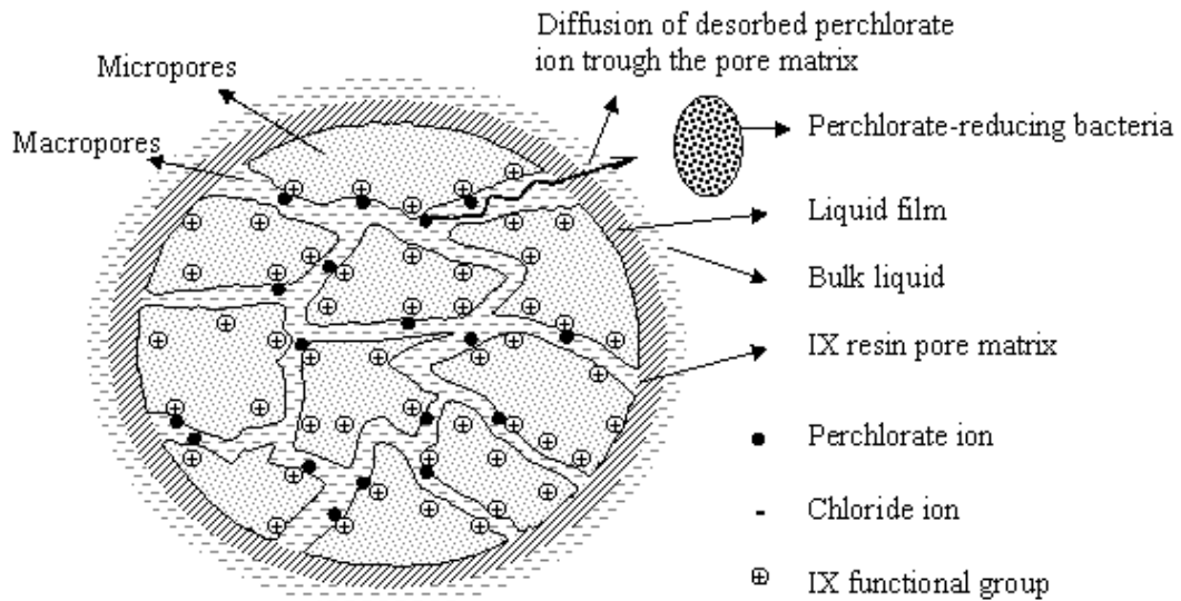
Figure 4.1. Conceptual Model for Biodegradation of Resin-attached Perchlorate in the Bioregeneration Process. It is envisioned that, to be biodegraded, RAP ions should: 1) Desorb from the functional group located in the resin bead matrix, 2) diffuse from the resin bead to the resin surface through the resin pores, 3) transfer through a liquid film on the resin surface to the bulk liquid, and 4) enter the periplasmic region of the PRB to be biodegraded.
