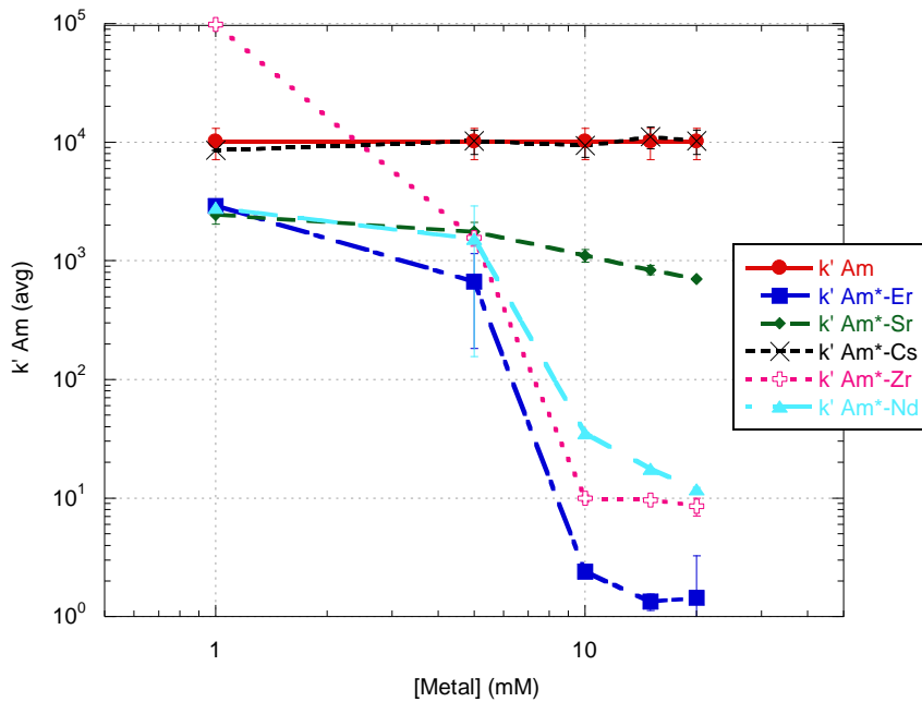
Figure 25. Used Fuel Component Effects on Am Adsorption to DGA resin in 1 M HNO_3
