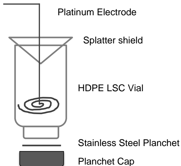
Figure 16. Electrodeposition Cell
