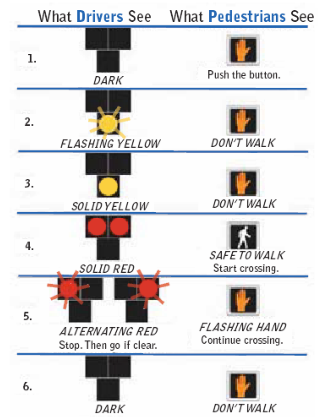
Figure 2-14. Pedestrian Hybrid Beacon System Operation (Fitzpatrick and Park, 2010)
