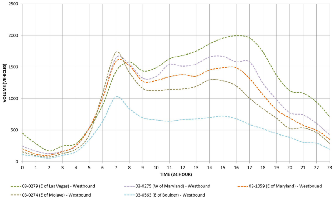
Graph 15: Sahara Avenue – Directional Distribution of Traffic (Westbound – East of Las Vegas Boulevard) AFTER
