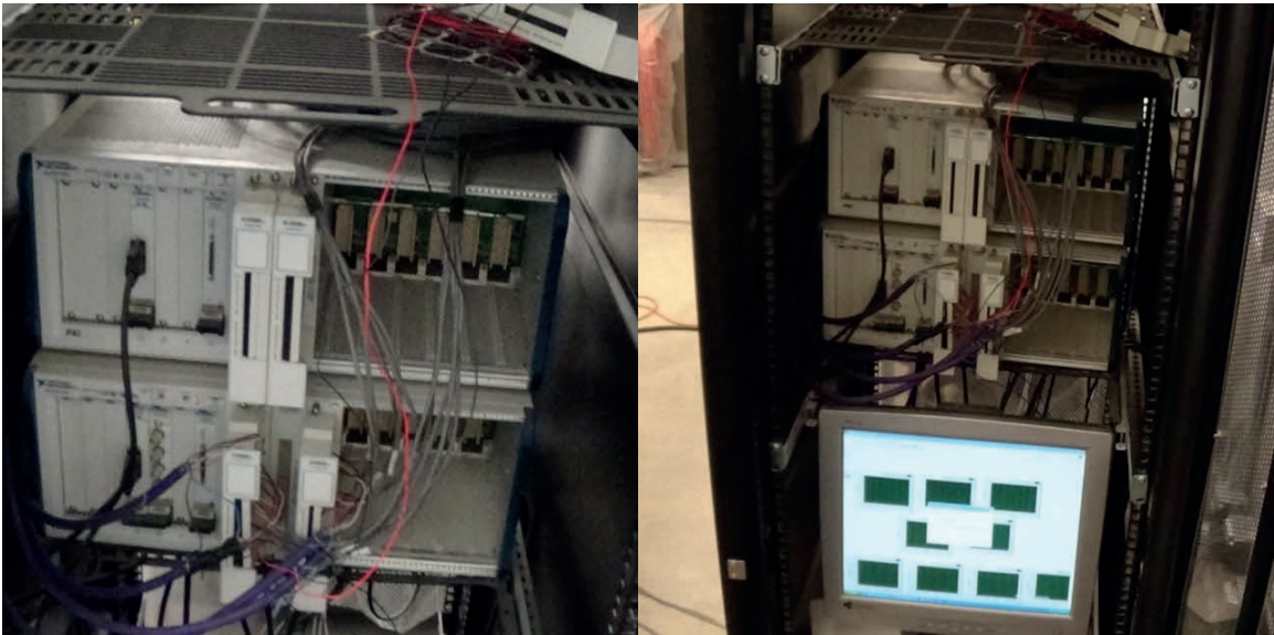
(a) (b) Figure 3.11: Data acquisition system
