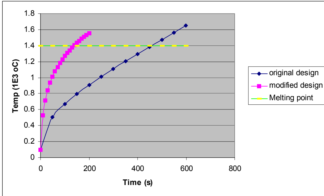
Figure 1.3.3. The time requirements for reaching the melting point using the different coil numbers.
