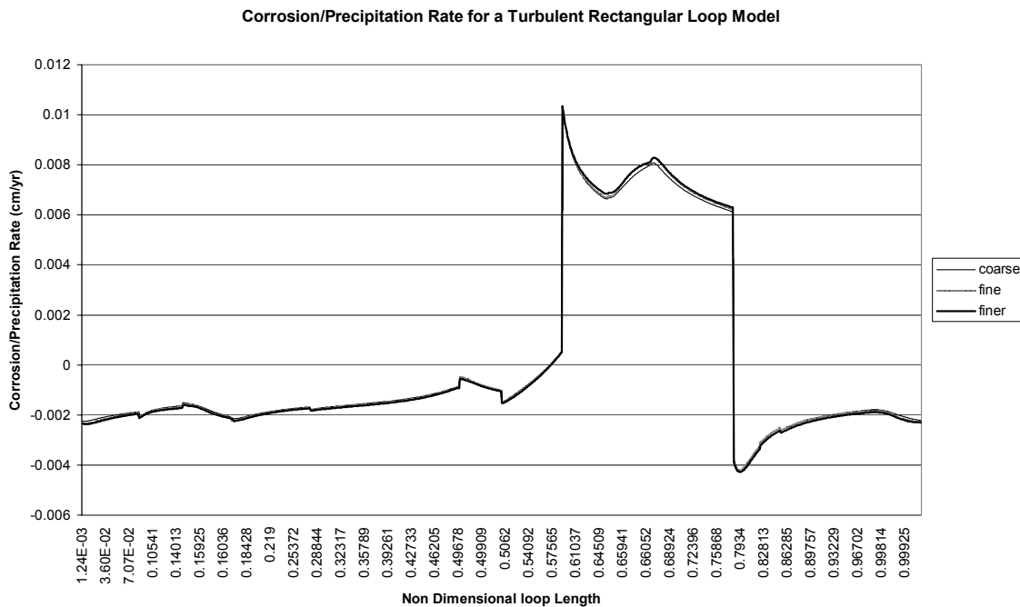
Figure 1.3.7. Grid Independency Check for a Turbulent Rectangular Loop Model
