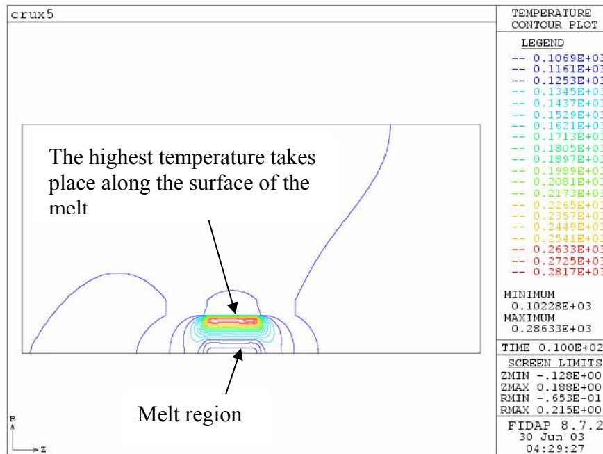
Figure 1.3.1. The temperature contours of induction heating furnace
