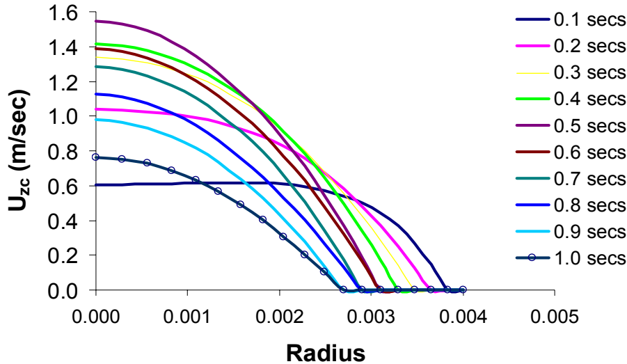
Figure 1.3.2. Axial velocity profile for constant inlet pressure of 20 kPa (mold preheated temperature=800 °C, inlet melt temperature=1,500 °C, interfacial heat transfer coefficient =2,000 W/m 2 °C).
