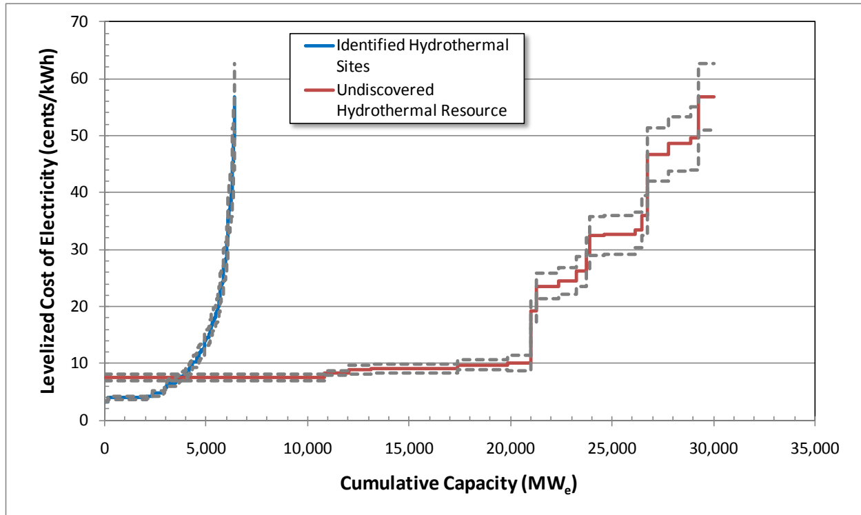
Figure 2: Supply curve for hydrothermal resource. Present-day median (50 th percentile) LCOE estimates in 2008 US$ from GETEM for identified and undiscovered resources. 10 th percentile and 90 th percentile values for each curve shown in gray.
