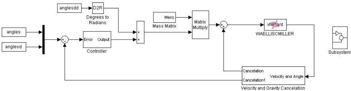
1 Computed Torque method implemented in MATLAB
