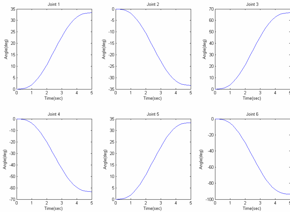
2 Joint angle responses after implementing the controller
