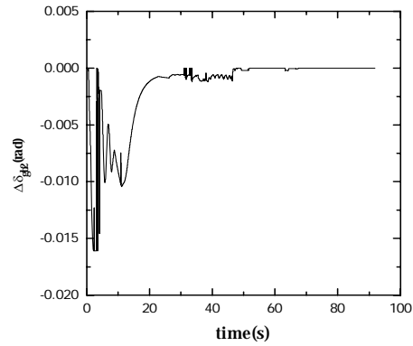
Fig. 29. Output of \Delta\delta_{gb2} .
