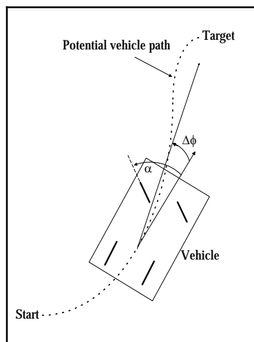
Fig. 4. Input Variables of the Target Steering Module.
