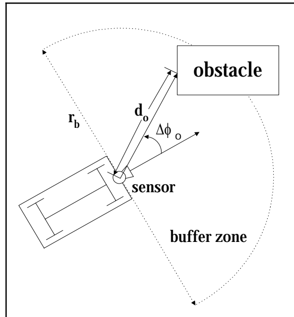
Fig. 2. Sensing Field Configuration.
