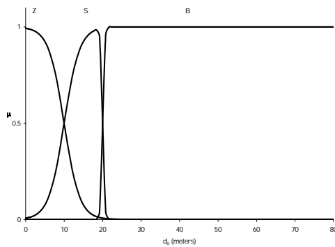
Fig. 7. Membership Functions for d_o .
