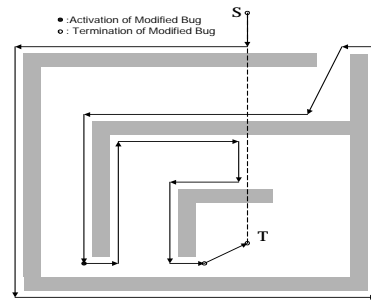
Fig. 11. Path 2 by Bug Steering Module.
