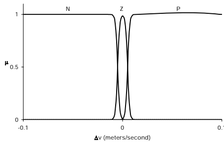
Fig. 19. Membership Functions for \Delta v .
