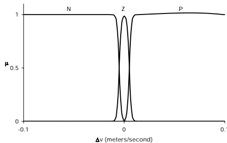
Fig. 19. Membership Functions for \Delta v .
