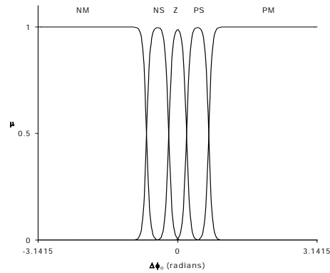
Fig. 8. Membership Functions for \Delta\phi .
