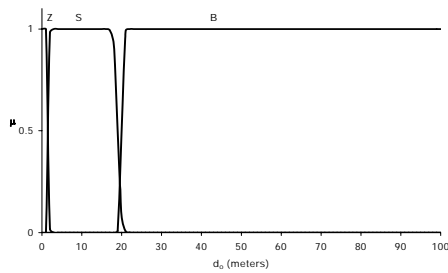
Fig. 23. Membership Functions for Input Variable, d_o .
