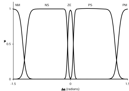
Fig. 14. Membership Functions for Output Variable \Delta\alpha_3 .
