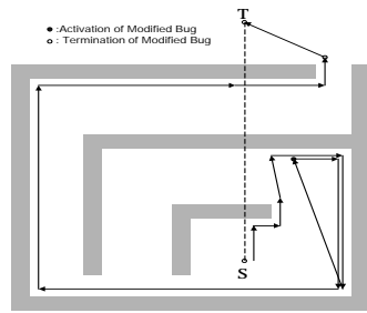
Fig. 10. Path 1 by Bug Steering Module.
