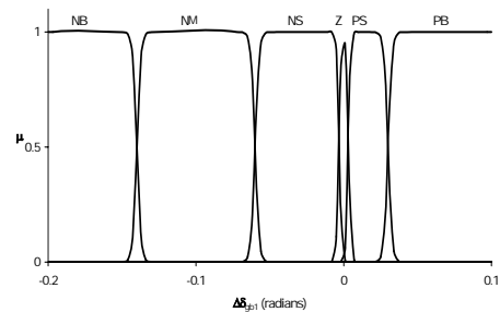
Fig. 20. Membership Functions for \Delta\delta_{gb1} .
