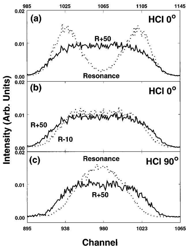
FIG. 10. \text{H}^+ peaks from HCl singles spectra. (a) Data taken on resonance (dotted line), and 50 eV above resonance (solid line) with the analyzer parallel to the polarization vector of the SR. (b) Data taken 10 eV below resonance (dotted), and 50 eV above resonance (solid) with the analyzer parallel to the polarization vector of the SR. (c) Data taken on resonance (dotted) and 50 eV above resonance (solid) with the analyzer perpendicular to the polarization of the SR. The labels on the top x axis correspond to the 0^\circ plots, while labels on the bottom axis correspond to the 90^\circ plot.
