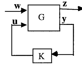
Fig. 1. Block diagram for nonlinear H_\infty formulation.
