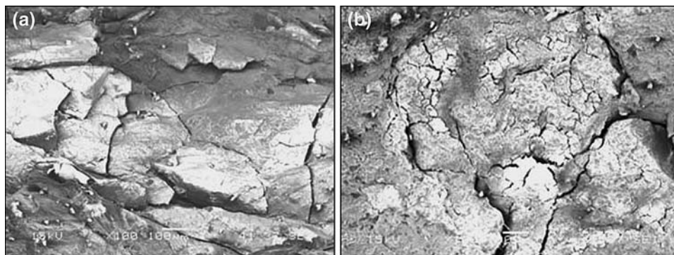
Fig. 8 SEM micrographs of convex surfaces of C-ring specimens. (a) 0.5 wt.% Si, 60 days, 100 \times (b) 2.0 wt.% Si, 60 days, 100 \times
