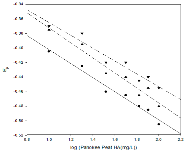
Figure 6. DPP results for Pb^{2+} at pH 8 plotted as a function of the log of the Pahokee peat humic acid concentration (mg/L) at three different concentrations of Pb^{2+} (● 1.61 \mu M, ▲ 4.82 \mu M and ▼ 9.63 \mu M).
