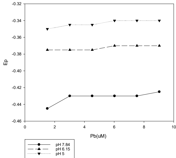
Figure 1. Differential pulse polarography (DPP) results for the reduction of Pb^{2+} in the presence of 1.25 mM 3,4-dihydroxybenzoic acid at three different pH values. The peak maximum ( E_p ) becomes increasingly negative as the pH increases.
