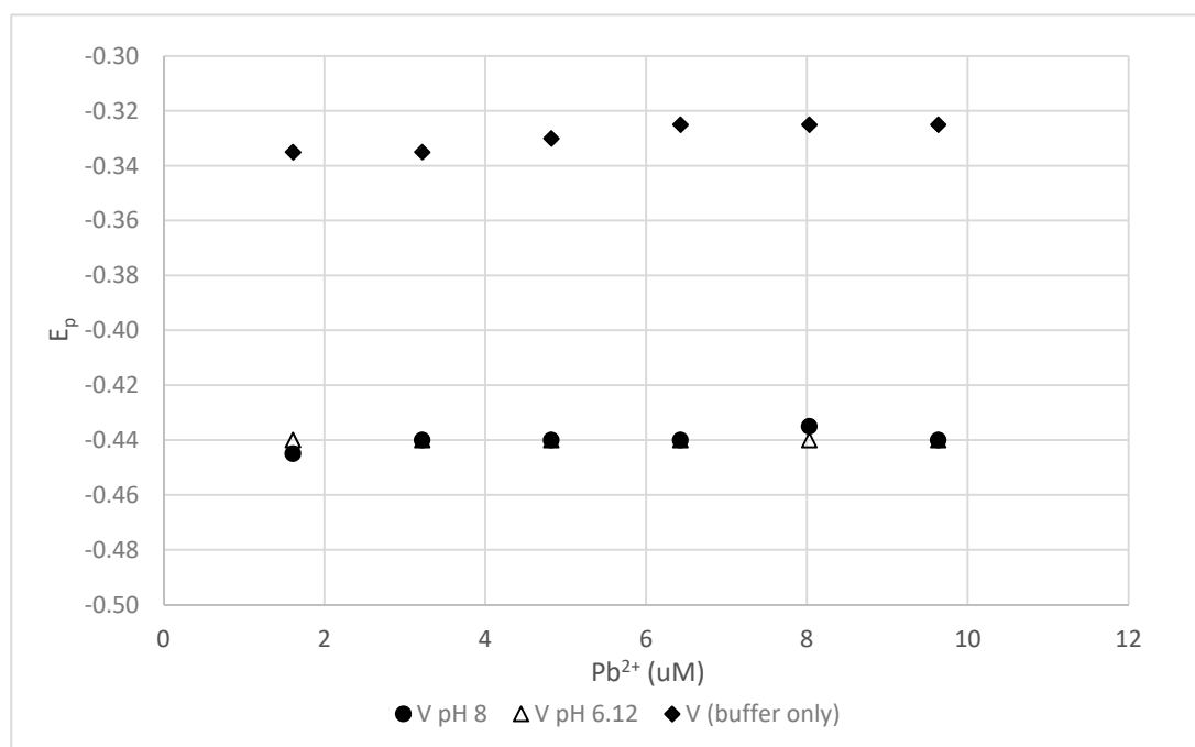
Figure 3. DPP results for \text{Pb}^{2+} in the presence of 100-mg/L polyacrylate. There is little difference in the results for pH 6.12 and pH 8.
