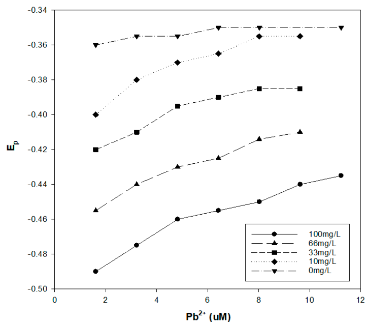
Figure 7. DPP results for Pb^{2+} at pH 8 in the presence of TeraVita leonardite humic acid. The E_p value shifts toward a more negative voltage with an increase in the humic acid concentration.
