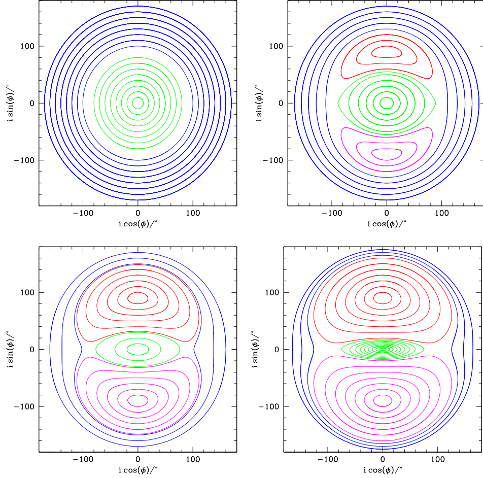
Figure 1. The i \cos \phi - i \sin \phi plane for misaligned test circular particle orbits with varying initial inclination and longitude of the ascending node. The green lines show orbits close to prograde, red/magenta lines show orbits that have a librating solution, and the blue lines show orbits close to retrograde. Upper left-hand panel: a circular binary with e_b = 0.0 . Upper right-hand panel: e_b = 0.3 . Lower left-hand panel: e_b = 0.6 . Lower right-hand panel: e_b = 0.8 .
