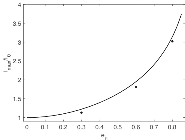
Figure 12. Plotted as a line is the maximum disc tilt as a function of binary eccentricity normalized by i_0 (defined in Fig. 11) based on equation (28). Plotted as dots are the results of SPH simulations for models Run6, Run7, and Run8 given in Table 2, which all have an initial circumbinary disc tilt i_0 = 10^\circ .
