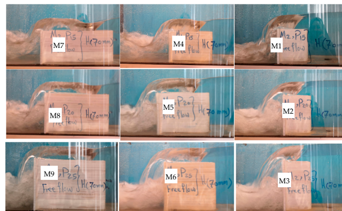
Figure 4. Photographs of the models, h = 70 mm.
