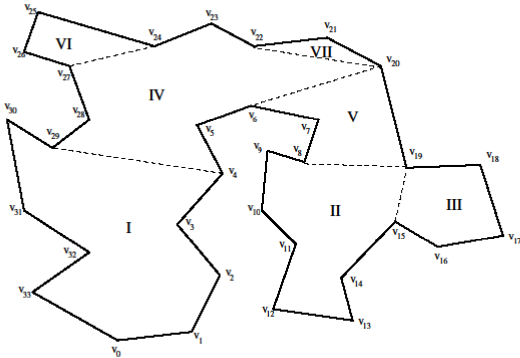
Figure 2.4 Polygon partitioned into monotone pieces – I, II, ... VII.
