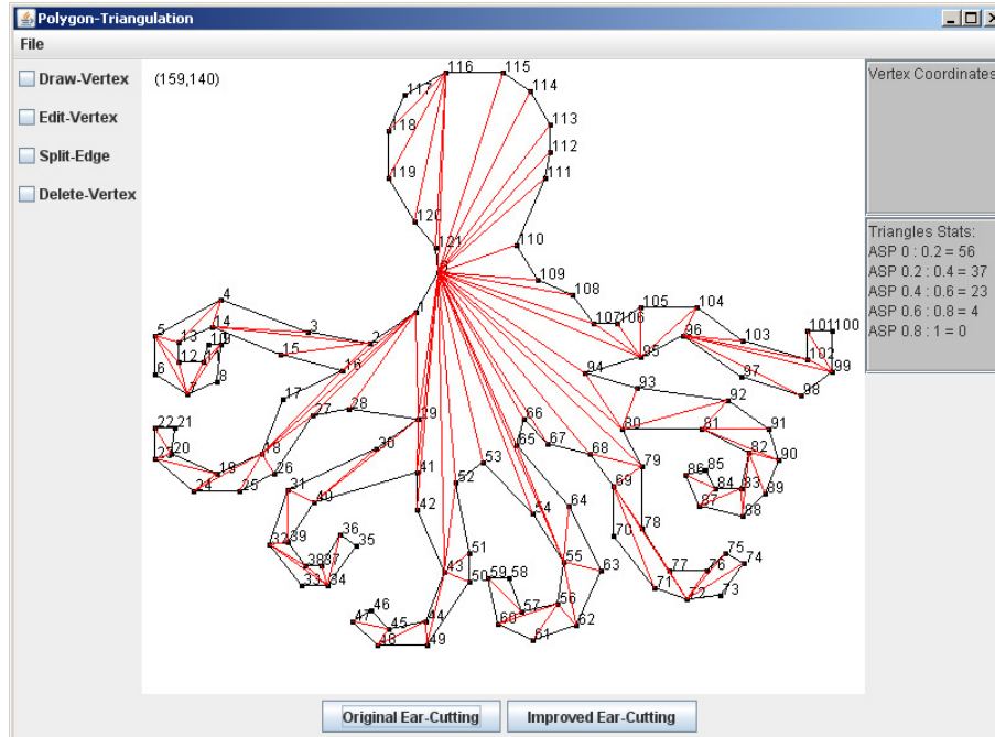
Figure 4.6: Figure triangulated using traditional ear-cutting method
